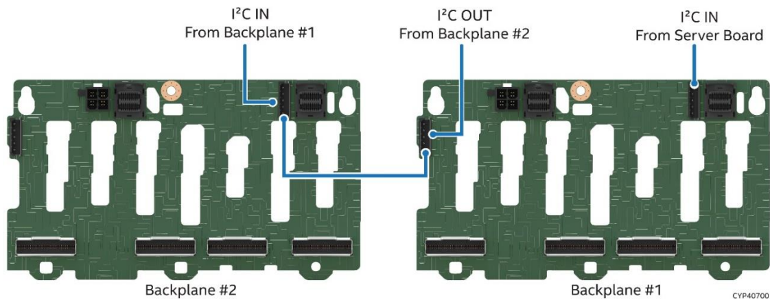
Figure 90. Connecting Two x8 Backplanes
