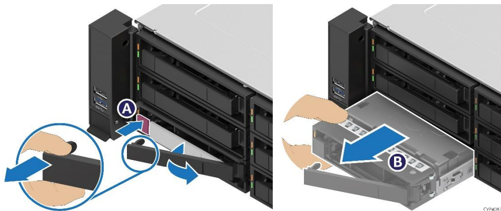
Figure 81. Drive Removal from 3.5" Drive Bay
