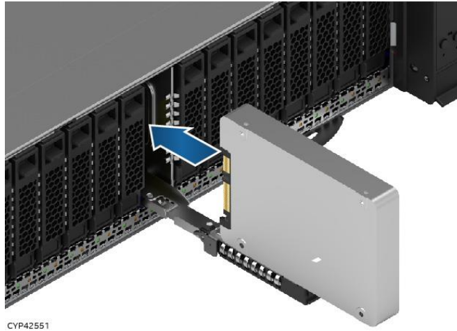
Figure 75. 15 mm Drive Insertion into 2.5" Drive Bay, Ready to Install
