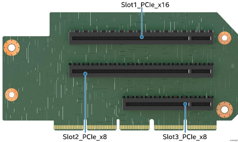
Figure 54. PCIe* Riser Card for Riser Slot #1
