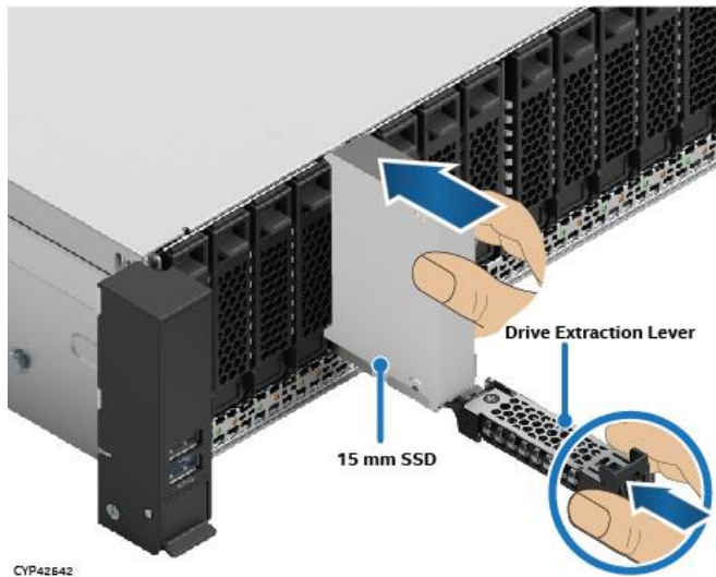
Figure 76. 15 mm Drive Insertion into 2.5" Drive Bay
