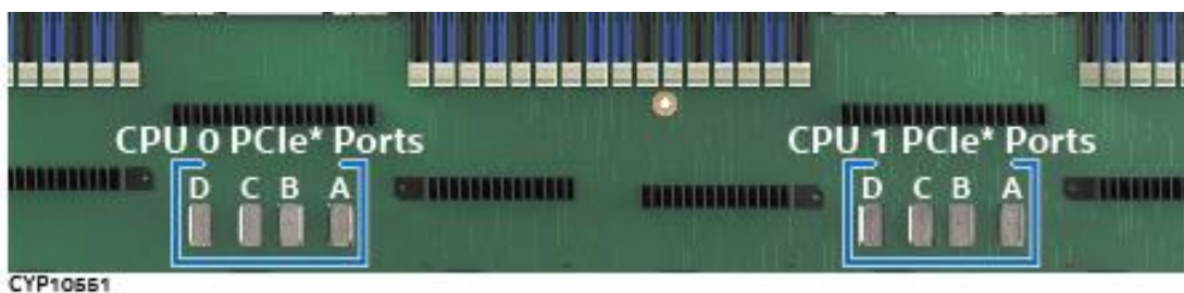
Figure 97. PCIe* SlimSAS* Connectors
