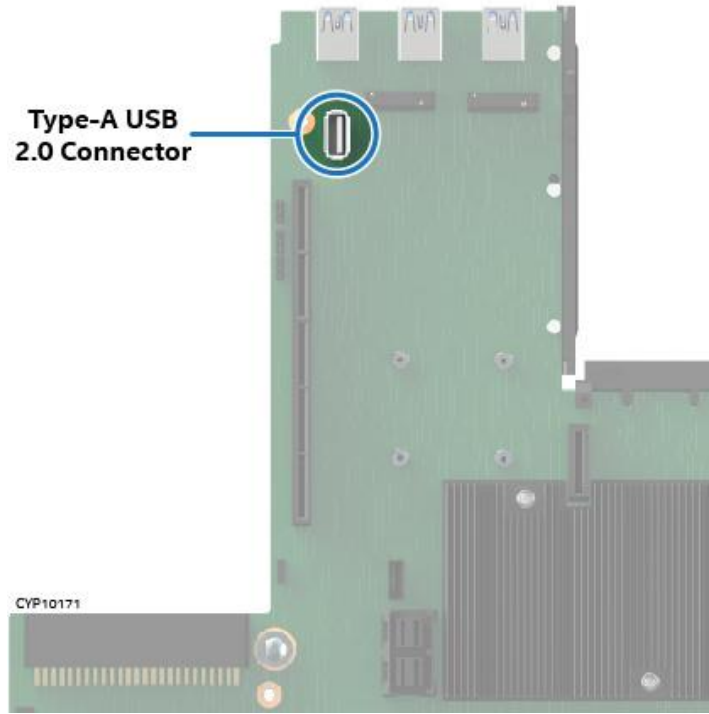
Figure 127. Internal USB 2.0 Type-A Connector
