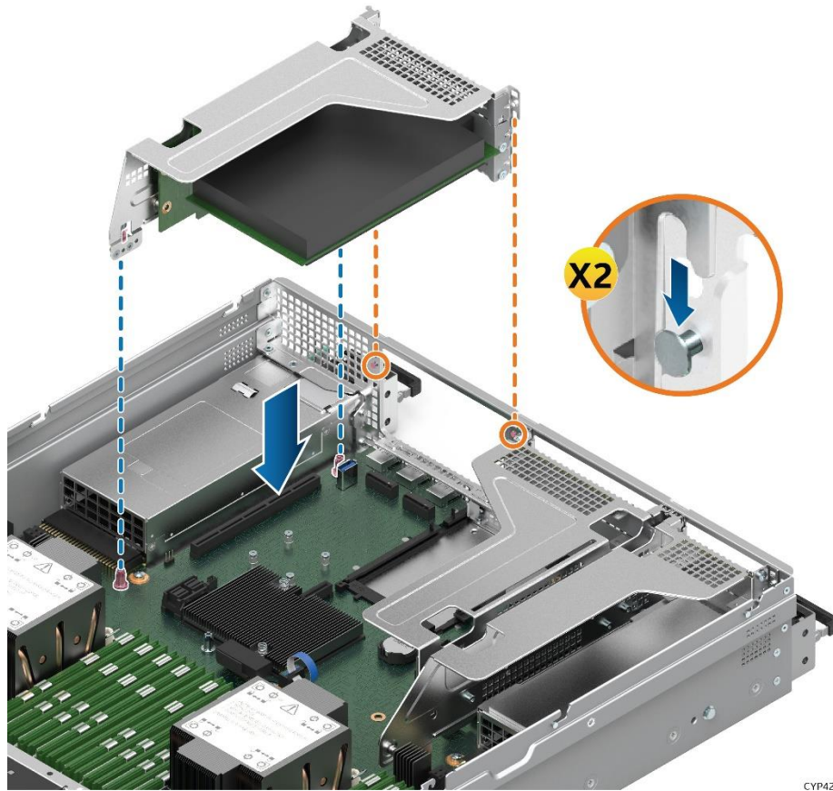
Figure 50. Add-in Card Placement into Server System Chassis
