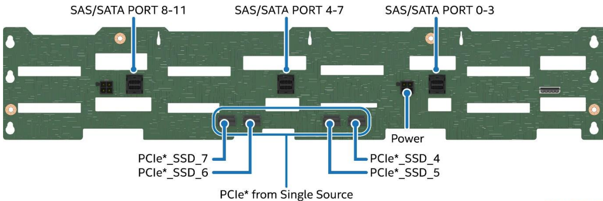
Figure 106. 12 x 3.5" HSBP Connector Identification – Back Side
